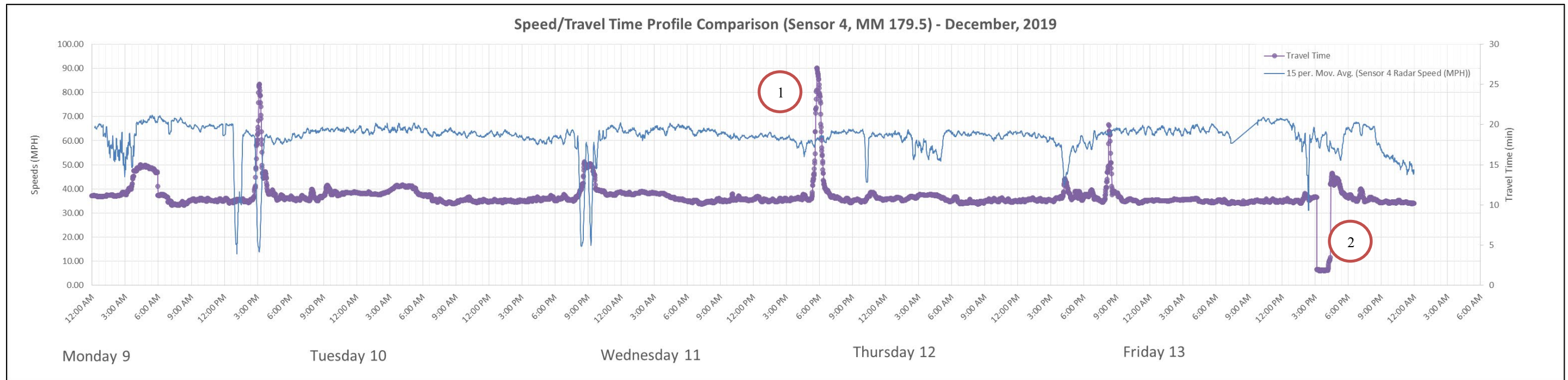
Figure 6. Data Accuracy Comparison Example (Sensor 4)
