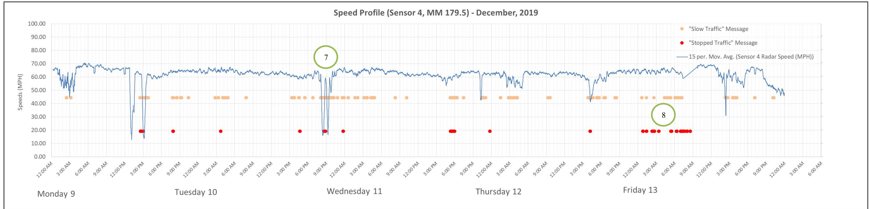
Figure 10. QWS Logic Review Examples (PCMS 3)
