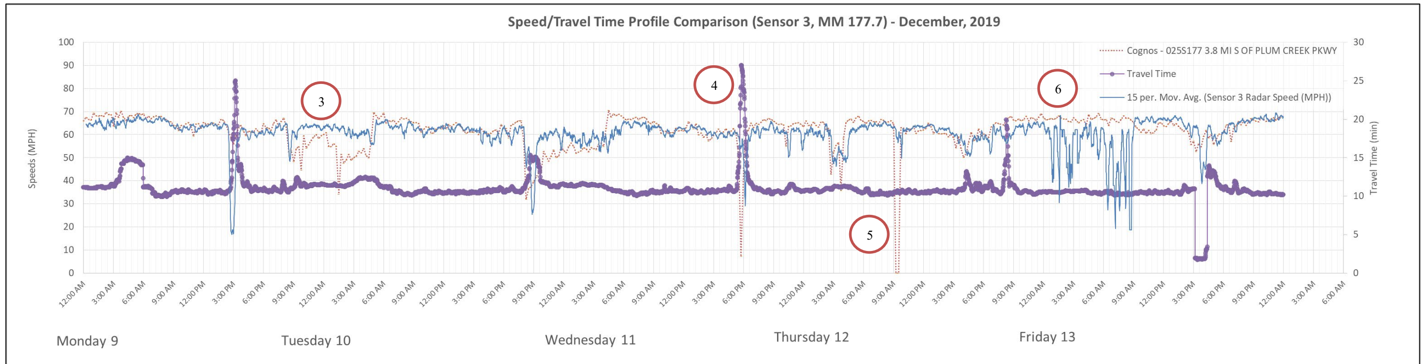
Figure 7. Data Accuracy Comparison (Sensor 3)
