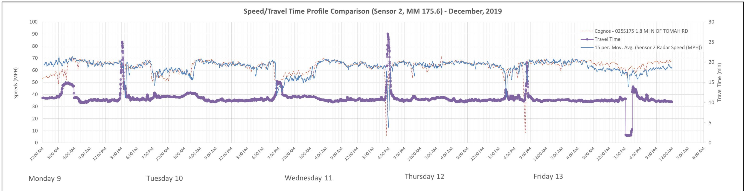
Figure 8. Data Accuracy Example (Sensor 2)
